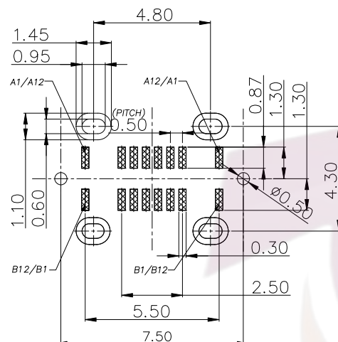
RECOMMENDED P.C.B. LAYOUT TOLERANCE UNSPECIFIED \pm 0.05\text{mm}
