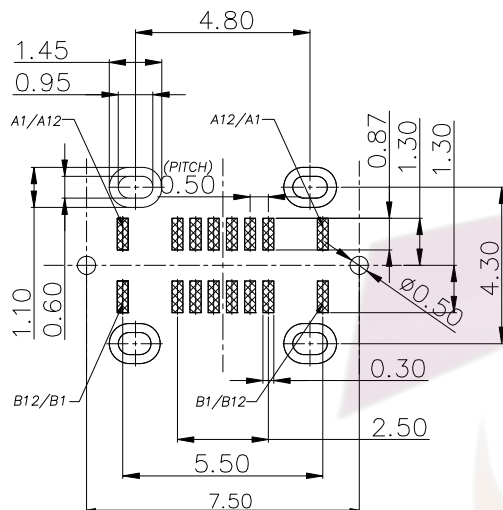
RECOMMENDED P.C.B. LAYOUT TOLERANCE UNSPECIFIED \pm 0.05\text{mm}
